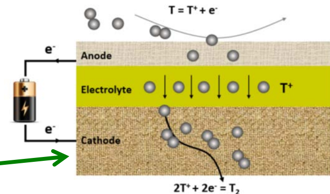
Schematic of INL's Proton Conducting Electrolytic membrane
