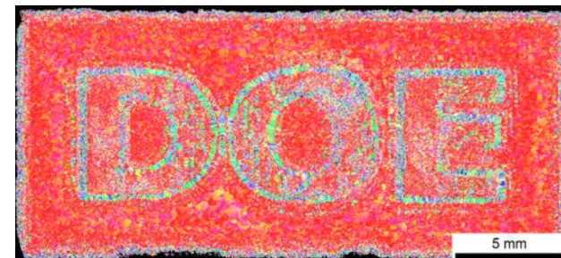
EBSD image of a nickel-based alloy showing designed microstructure orientation created by an AM machine at ORNL
