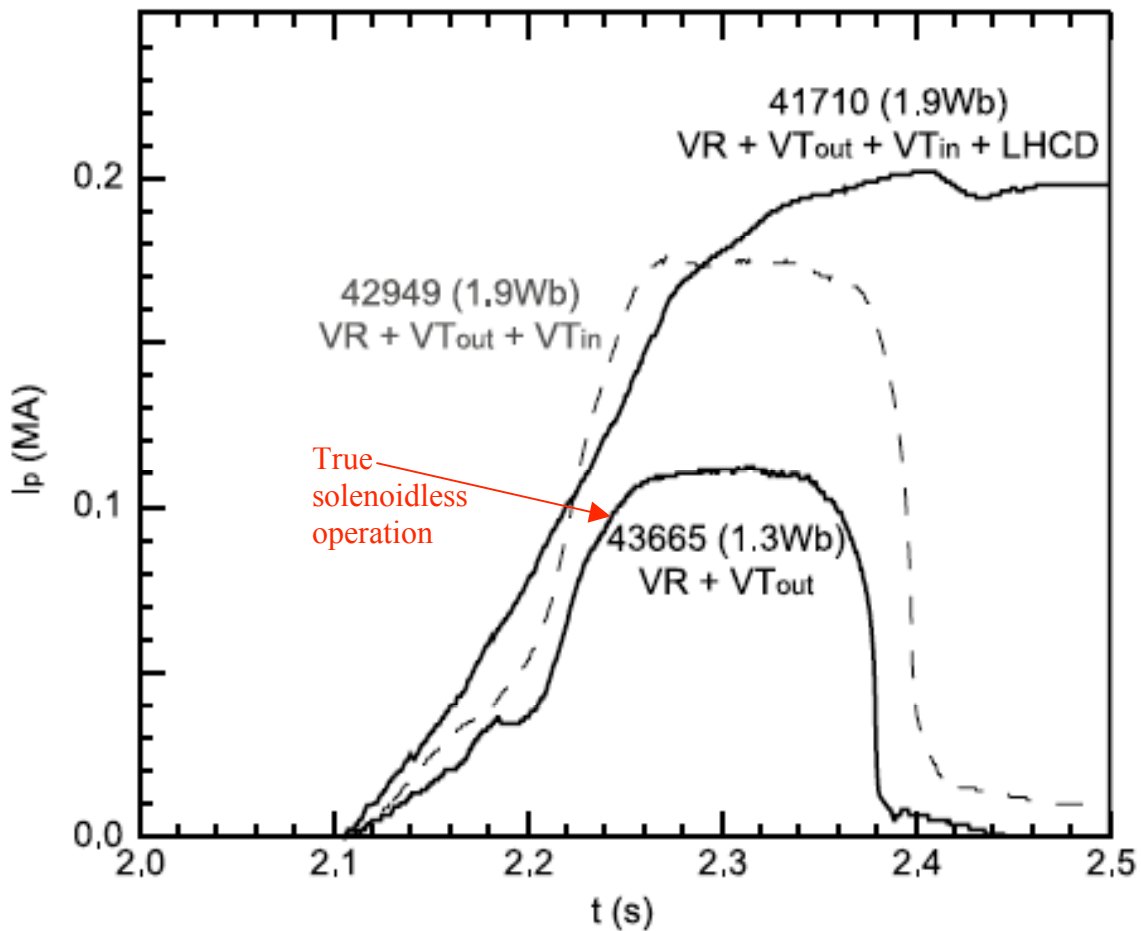
Figure 1 . JT-60U Solenoidless I_p start-up. Shot 43665 uses outside PF coils only and ~1MW ECH to achieve 100kA and is truly a solenoidless startup. Other discharges used a partial solenoid for startup. 41710 used LHCD to achieve further I_p rampup. [2]
