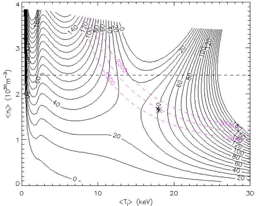
Figure 2. ARIES-AT popcon showing nominal operating point (asterisk) on high temperature side of contour. Confinement is scaled from ITER-89P with H_{90}=2.65 .
